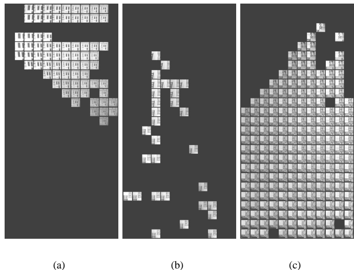
Fig. 9. Typical examples of feature visibility regions obtained after executing the feature matching algorithm in [40].
